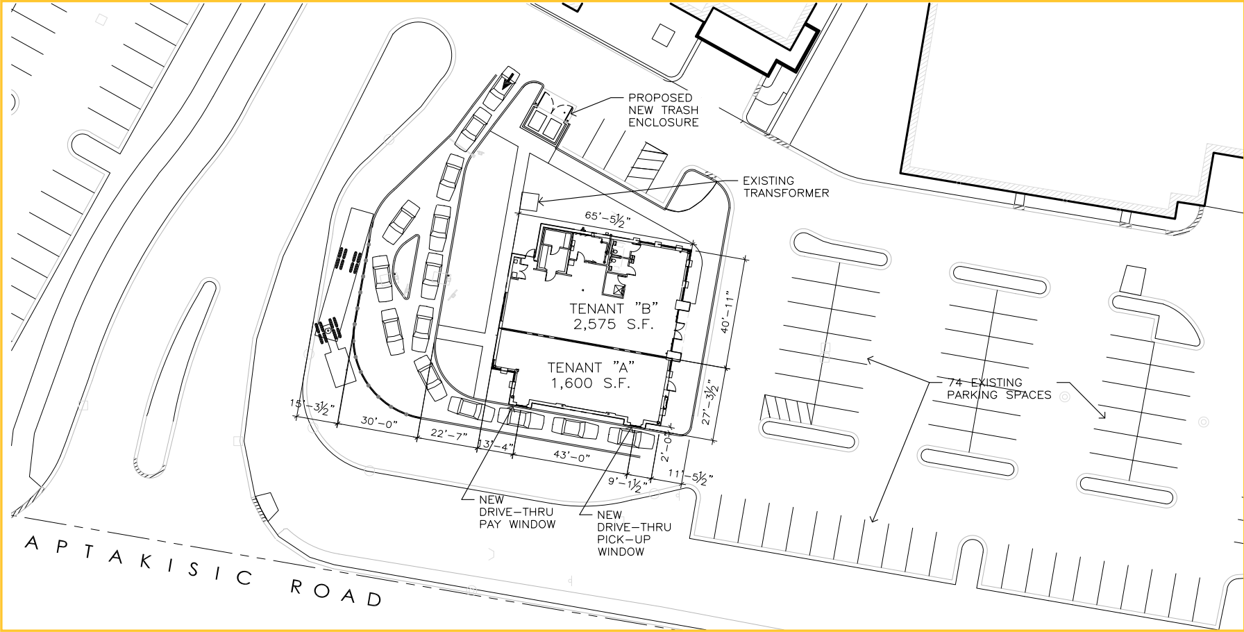
Proposed Demising Plan
